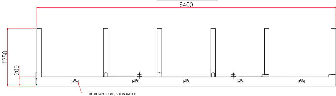
SIDE VIEW
