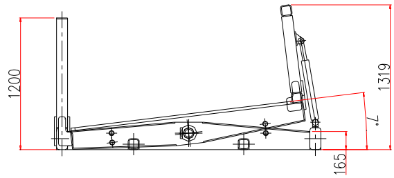
FRONT VIEW , BIN TILTED
